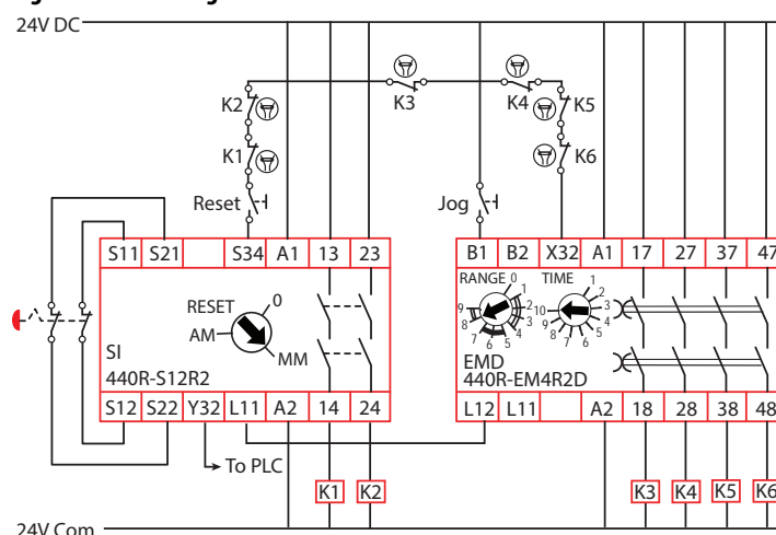
Figure 48 - EMD - Jog
