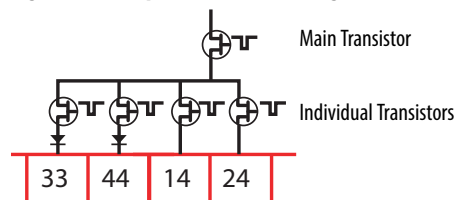
Figure 27 - Output Transistor Arrangement
