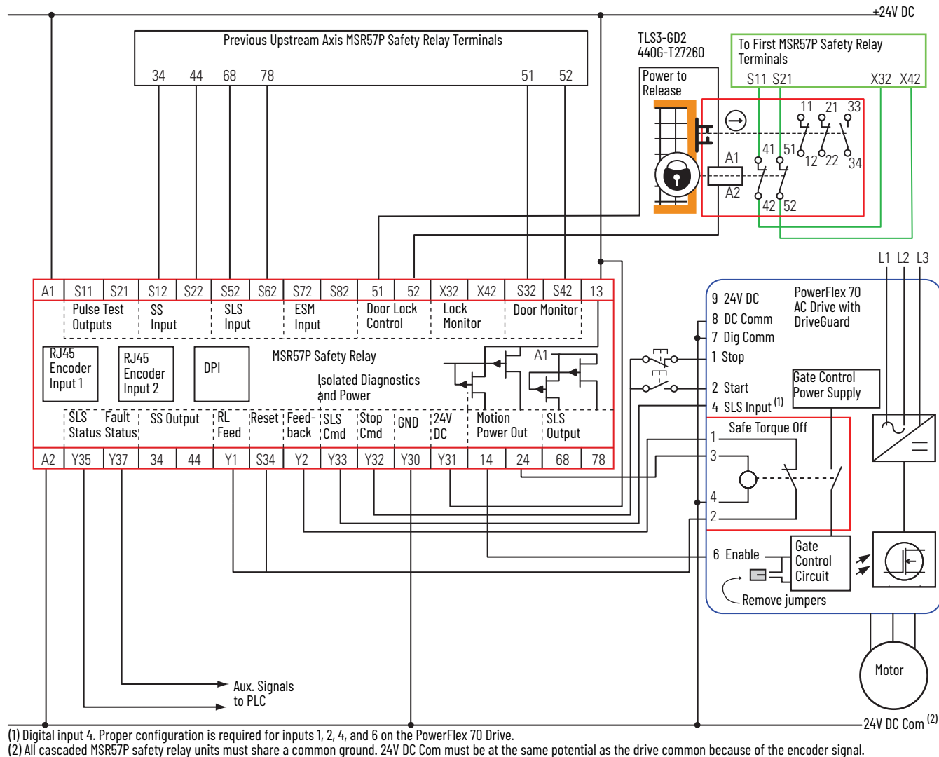
Figure 29 - Slave, Safely-limited Speed, Last Unit
