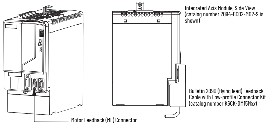
Integrated Axis Module, Front View (catalog number 2094-BC02-M02-S is shown)
