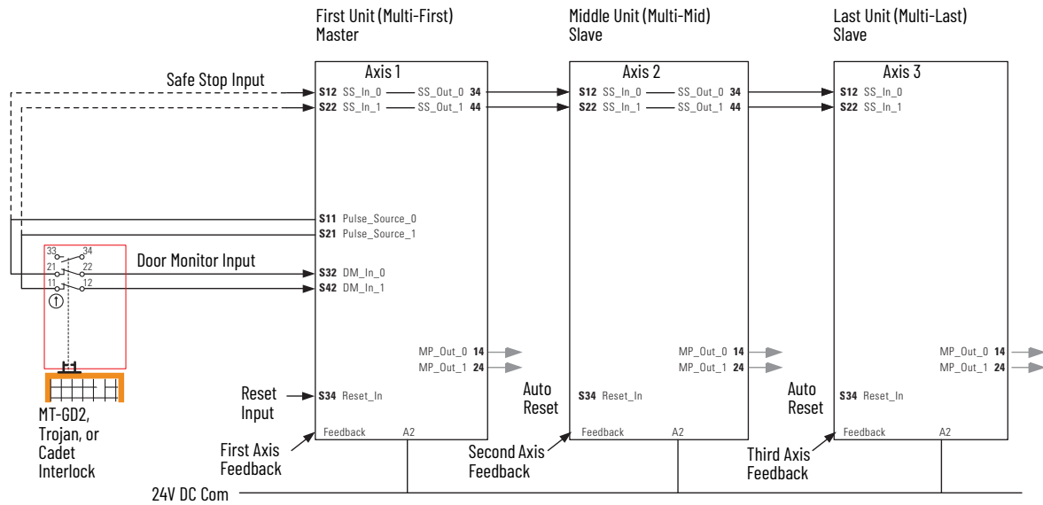
Figure 35 - Safe Stop and Safely-limited Speed with Door Monitoring (5-wire) Connections
